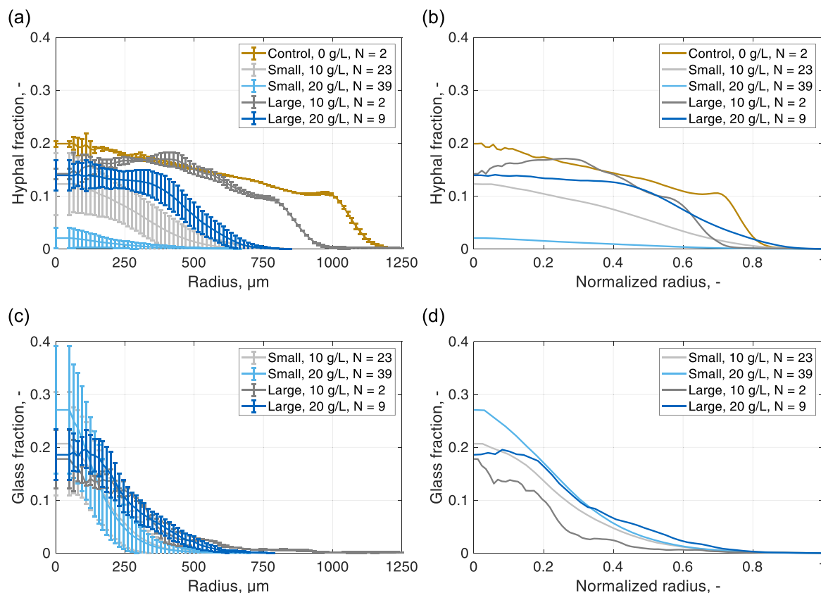
FIGURE 9 (a) Mean hyphal fractions over the pellet radius and (b) mean hyphal fractions over the normalized pellet radius. (c) Corresponding mean glass fractions over the pellet radius and (d) mean glass fractions over the normalized pellet radius with small and big microparticle at a concentration of 10 and 20 g/L. The data points are mean values calculated with the pellet sample number (N) per cultivation. The error bars indicate the standard deviation between the pellets of the same sample. To obtain the normalized radius of each pellet, the distances to the pellet center were divided by the maximum distance, which corresponded to the maximum radius of the respective pellet. The measured values were then linearly interpolated to obtain equal spacing for the pellets compared with each other.
